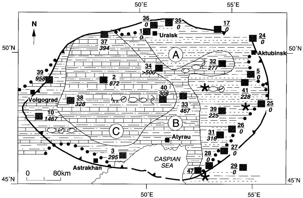
FIG. 12. — Upper Triassic lithological and palaeogeographical scheme of the Precaspian Depression. A , alluvial plain, flooded episodically by the sea; B , C , carbonate-clastic ( B ) and clastic-carbonate ( C ) deposits of shallow epicontinental sea. Legend: see Fig. 7. List of boreholes: 1, Vetekin; 2, Aralsor; 3, Zhambay; 5, Karabulak; 10, Sadovaya; 17, Mertvye Soli; 24, Jusa; 25, Zhanazhol; 26, Chikembay; 27, Mashly; 28, Suishbek; 29, Chumyshty; 31, Zhusalysay; 32, Chobda; 33, Matenkozka; 34, Kusankuduk; 35, Pavlov; 36, Teplov; 37, Ershov; 38, Shungay; 39, Novonikol; 40, Inder; 41, Shubarkuduk; 47, East Prova.
