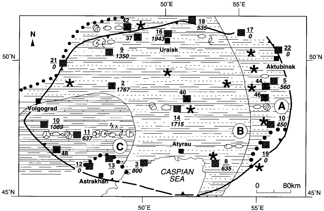
FIG. 10. — Lower Triassic lithological and palaeogeographical scheme of the Precaspian Depression. A, area of alluvial and proluvial deposits; B, alluvial plain, flooded episodically by the sea; C, epicontinental marine deposits. Legend: see Fig. 7. List of boreholes: 2, Aralsor; 3, Zhambay; 5, Karabulak; 8, Kulsary; 9, Kurilov; 10, Sadovaya; 11, Bugrin; 12, Stepnov; 13, Zavolzh; 14, Ushtobe; 16, Chinarev; 17, Mertvye Soli; 18, Akzhar; 19, Tuskum; 21, Nikolaev; 22, Podgornen; 37, Ershov; 40, Inder; 42, Eruslan; 44, Kenkiyak; 46, Biaktykol; 48, Shar-Tsaryn.
