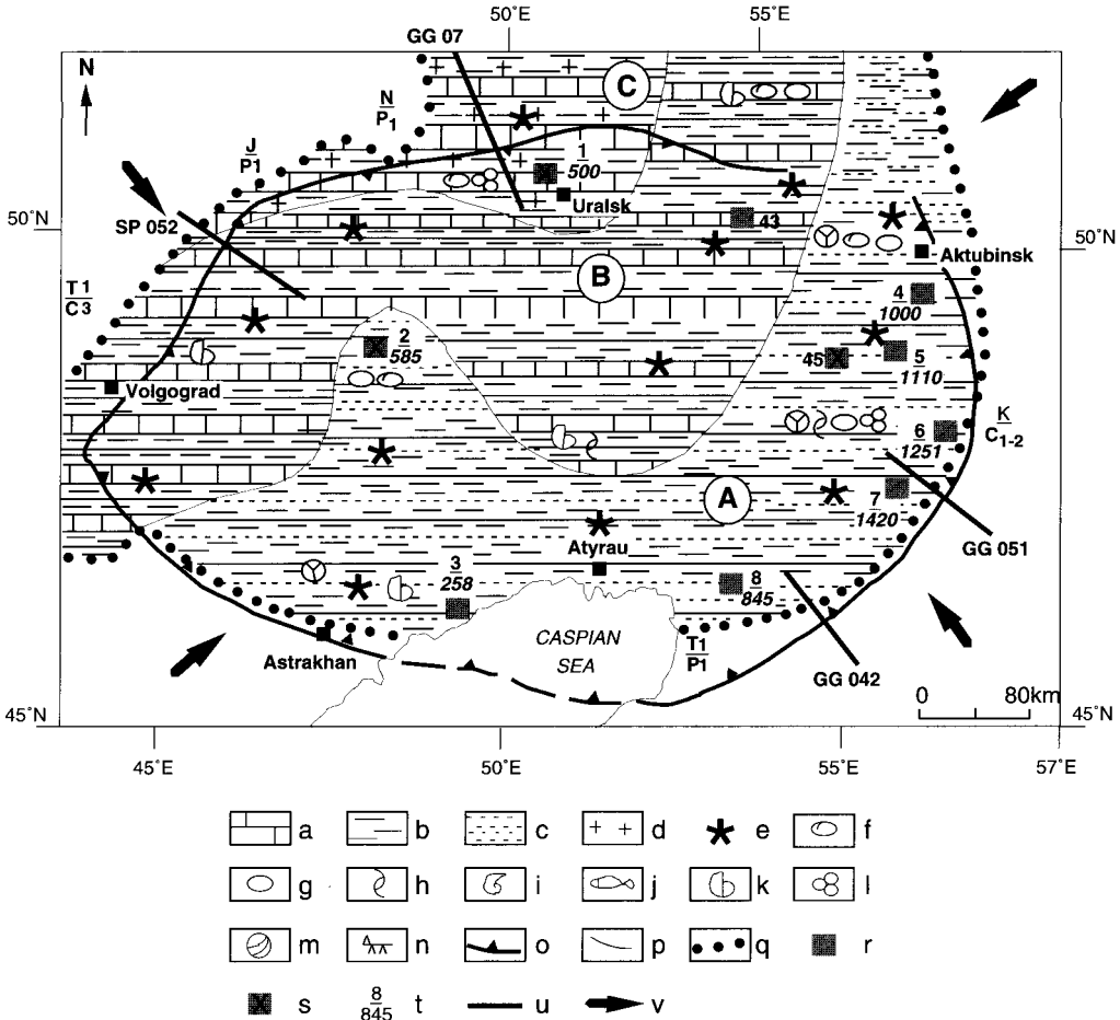
FIG. 7. — Kazanian lithological and palaeogeographical scheme of the Precaspian Depression. A , alluvial plain episodically flooded by the sea; B , C , area of marine (during lower Kazanian-kz1) and lacustrine (during upper Kazanian-kz2) carbonate-clastic ( B ) and salty carbonate ( C ) deposits. Legend for all the palaeogeographic maps: a , carbonates; b , shales; c , sandstones; d , salt; e , redding; f , marine ostracods; g , non-marine ostracods; h , pelecypods; i , cephalopods; j , fishes; k , brachiopods; l , foraminifera; m , charophytes; n , vertebrates; o , Precaspian Basin boundaries; p , limits of lithological-palaeogeographical domains; q , limits of recent deposit abundance; r , boreholes; s , boreholes figured on figs 6, 8, 9, 11; t , number of boreholes (in the upper part number of the borehole; in the lower part, in italic, thickness); u , cross section of Figs 2-5; v , direction of detrital supplies. List of boreholes: 1, Vetekin; 2, Aralsor; 3, Zhambay; 4, Sambay; 5, Karabulak; 6, Kokzhide; 7, Mujunkum; 8, Kulsary; 43, Linevka; 45, Lugov.
