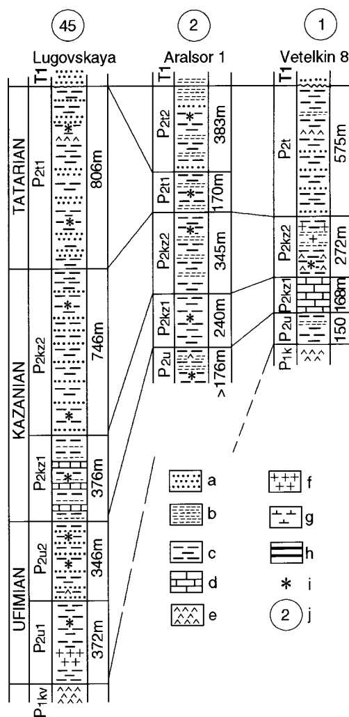
FIG. 6. — The Upper Permian of the Precaspian Depression illustrated by some representative boreholes (Lugovskaya 1, 45 on Fig. 7; Aralsor 1, 2 on Fig. 7; Vetelkin 8, 1 on Fig. 7). Legende: a, sand, sandstone; b, siltstone; c, shale; d, limestone; e, anhydrite; f, salt; g, carbonated shale; h, coal; i, red rocks; j, number of boreholes on palaeogeographic maps (Figs 7, 10, 12).
