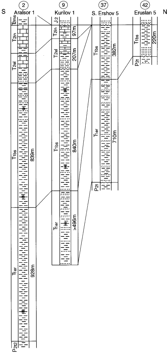
FIG. 9. — The Lower Triassic of the Precaspian Depression illustrated by some representative boreholes (Aralсор 1, 2 on Fig. 10; Kurilov 1, 9 on Fig. 10; South Ershov 5, 37 on Fig. 10; Erulsan 5, 42 on Fig. 10). Legend: see Fig. 6.
