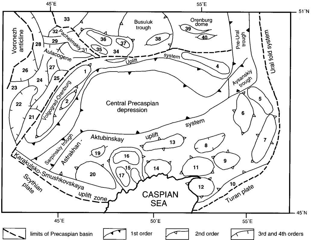
Fig. 1. — Tectonic chart of the Precaspian Depression. Tectonic features: 1, Akhtubinsk-Palassowski megamound; 2, Dzhanibeckoe rise; 3, Altatinsk-Nikolskiy mound; 4, Karachaganak-Koblandinskay uplift; 5, Temirskiy dome; 6, Kzyldsharskiy dome; 7, Zharkamysskiy dome; 8, Dossorskiy trough; 9, Bilkhalskiy dome; 10, South Emba uplift; 11, Guriev dome; 12, Karaton-Tengiz uplift; 13, Zhaykyskiy dome; 14, North-Caspian dome; 15, Akkolskiy dome; 16, Myntobinskay uplift; 17, Kobyakovskoe uplift; 18, Otyabrskoe uplift; 19, Azgirske uplift; 20, Astrakan dome; 21, Suvodskaya uplift; 22, Olkhovskay depression; 23, Archedino-Don mound; 24, Zhirnovsko-Umetovskiy mound; 25, Antipovsko-Sherbakovskiy mound; 26, Tersinskaya depression; 27, Zolotovsko-Kamenskaya uplift; 28, Karamyshskaya uplift; 29, Elshano-Sergievskiy mound; 30, Stepnovskiy mound; 31, Voskeresenskaya depression; 32, Saratov displacements; 33, Kazanlinskiy mound; 34, Pugachevskiy dome; 35, Marievskaya uplift; 36, Balakovskaya uplift; 37, Klintsovskay uplift; 38, Kamelik-Chaganskiy mound; 39, Zemlyanskiy mound; 40, Syrtovskiy mound.
