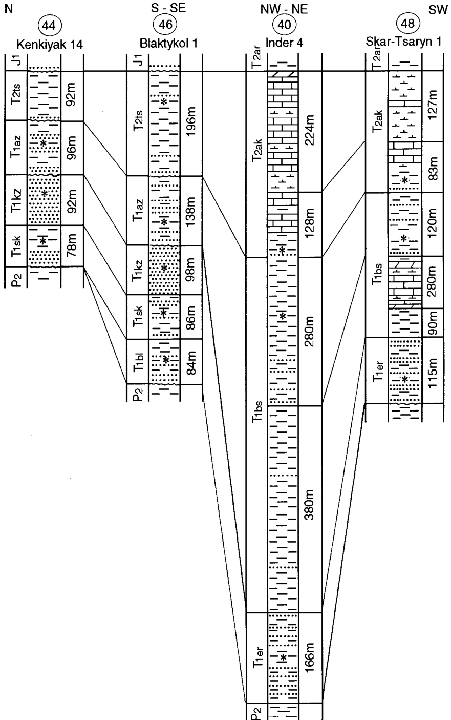
FIG. 8. — The Lower and Middle Triassic of the Precaspian Depression illustrated by some representative boreholes (Kenkiyak 14, 44 on Fig. 12; Blaktykol 1, 46 on Fig. 12; Inder 4, 40 on Fig. 12; Skar-Tsaryn 1, 48 on Fig. 12). Legend: see Fig. 6.
