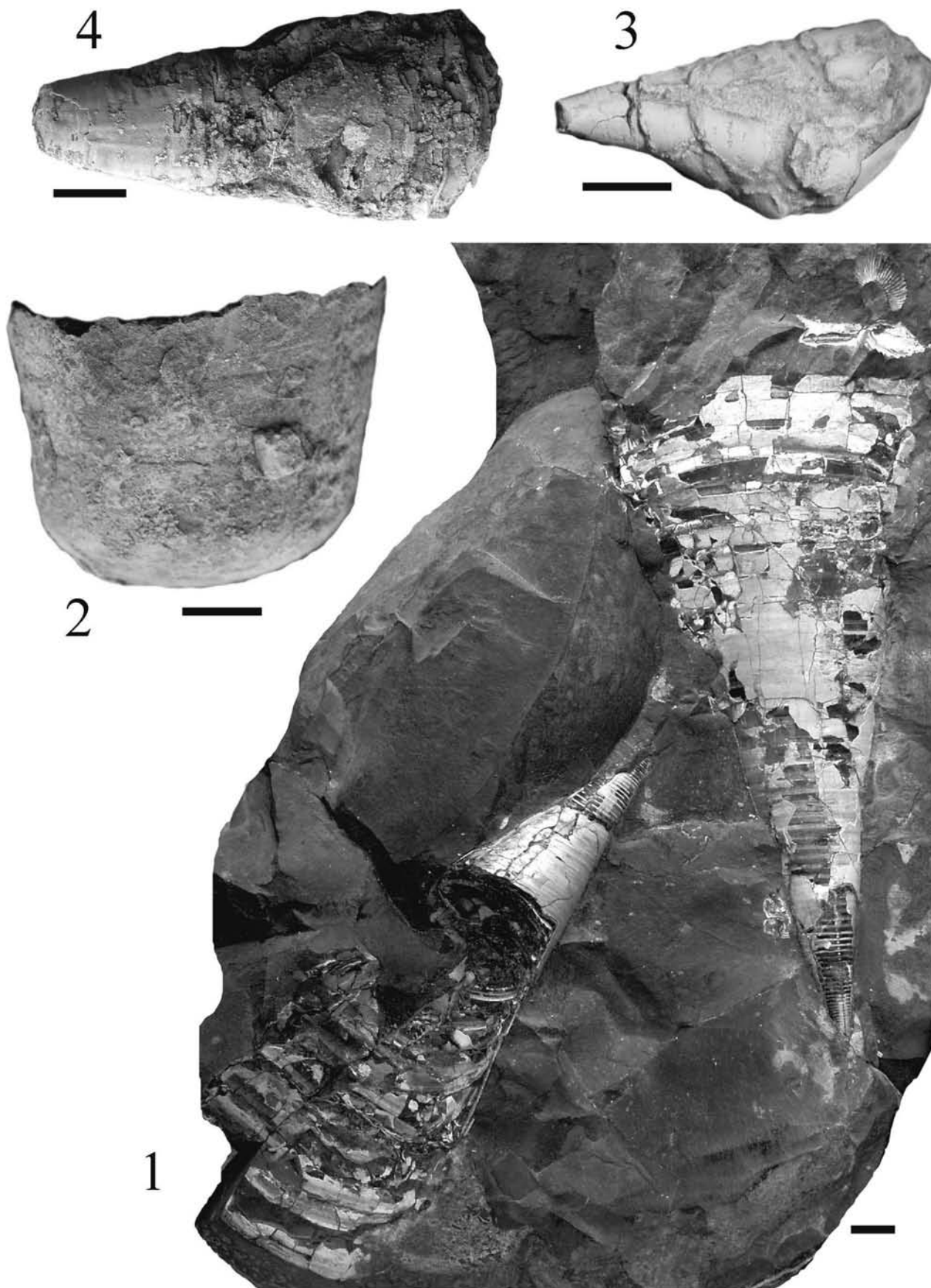
Plate 1. Callovian Belemnitoides. 1. Volgobelus sp., UPM, specimen without number, Prosek-Isady; Lower Callovian, Elatmae Zone, elatmae horizon (collected by V. M. Efimov). Orientation of the left shell is not clear; right shell is facing ventral side up. 2. Volgobelus (?) sp. Phragmocone; dorsal view. GIN MK1758, Perchem, Lower Callovian, Gracilis Zone, Michalskii Subzone, bed 13 after Rogov et al., 2002. 3. Acanthoteuthis sp. GIN MK1416, Stoilensk mine, Lower Callovian, ?Elatmae Zone (not in situ), pyrite mould. 4. Acanthoteuthis antiqua (Pearce). Dorsal view of the phragmocone; anterior end on the right. GIN MK1763, Dubki, Upper Callovian, Lamberti Zone, praelamberti horizon. Scale bars = 1 cm.
