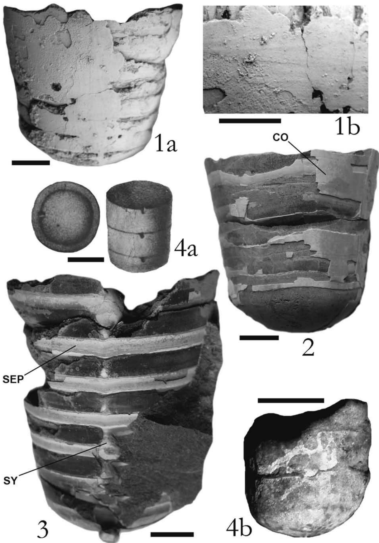
Plate 4. Middle Volgian to Barremian Belemnotheutids. 1. ?Acanthoteuthis sp., GIN MK1759, Glebovo, Middle Volgian Nikitini Zone (collected by D. N. Kiselev), a – general view; b – details of the conotheca sculpture showing longitudinal ornament; 2, 3. Volgobelus sp., Ryazanian-Valanginian of Bojarka river basin, not in situ (collected by A. S. Savitsky), 2 – GIN MK 1754, dorsal view; 3 – GIN MK1755-1, ventral view; 4. Acanthoteuthis (?) sp., Biassala, Crimea, Lower Barremian (collected by E. Eichwald), a – refigured sketch from Eichwald, 1865–1868, pl. XXXII, fig. 15; b – original specimen of Eichwald, SPbSU 2/2039. Abbreviations: CO – conotheca; SEP – septa; SY – siphuncle. Scale bars = 1 cm.
