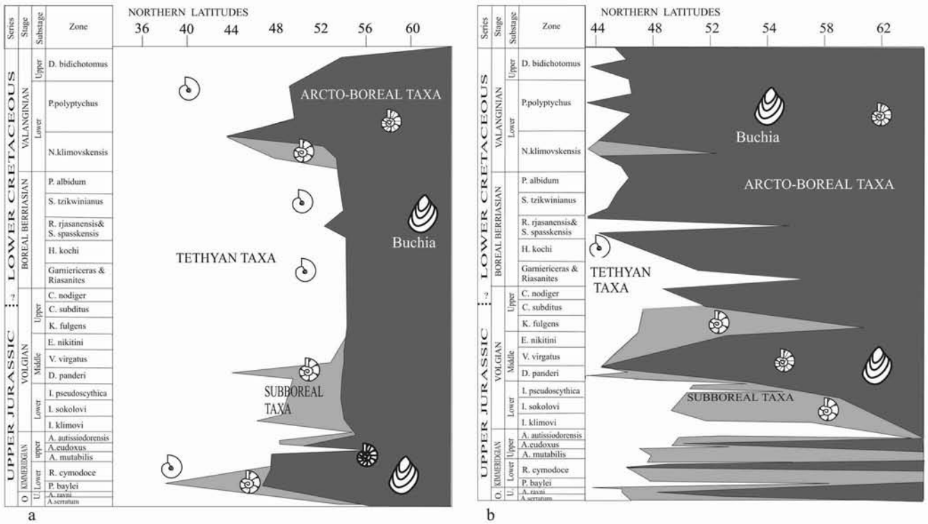
Fig. 3 - Molluscs migration restricted by the ecotone in the Boreal-Atlantic Realm from Kimmeridgian to Valanginian. a) West-European Province; b) East-European Province.
