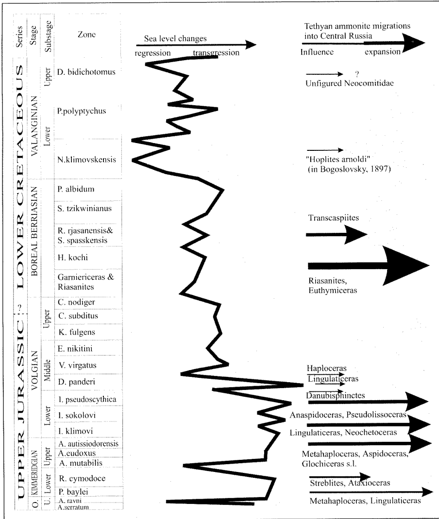
Fig. 4 - Transgressive-regressive curve (from Sahagian et al. 1996) and ammonite migrations into Central Russia (from Sahagian et al. 1996) and ammonite migrations via the Middle Russian Sea during the Kimmeridgian-Valanginian.
