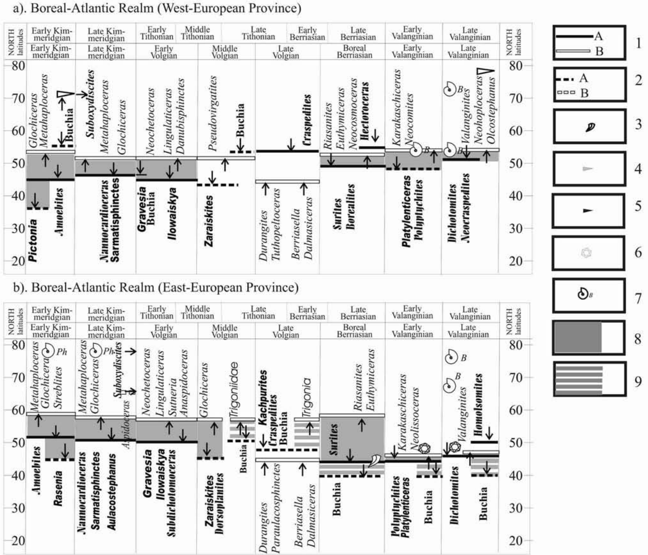
Fig. 2 - Setting of the Boreal-Tethyan ecotone and boundary between Boreal and Tethys-Pantalassa Super-realms from Kimmeridgian to Valanginian. 1-2 – Boreal (A) and Tethyan (B) expansions (1) and isolated straying (2); 3 – finds of Rudista together with Boreal ammonites; 4 – finds of Tethyan belemnites ( Hibolites ) together with boreal ammonites; 5 – finds of hermatypic corals together with boreal ammonites; 6 – oceanic ammonites in the high latitudes (Ph – Phyllocerata; L – Lytocerata; B – Bochianites ); 7 – ecotone based on ammonoids; 8 – ecotone based on ammonites and bivalves or only on bivalves. Affiliations of ammonites and bivalves noted by different fonts. Ammonites: Tethyan Glochiceras , Boreal with Tethyan affinities Suboxydiscites , Sub-boreal Zarisaites , Boreal Surites . Bivalves: Boreal Buchia , Tethyan Trigonidae .
