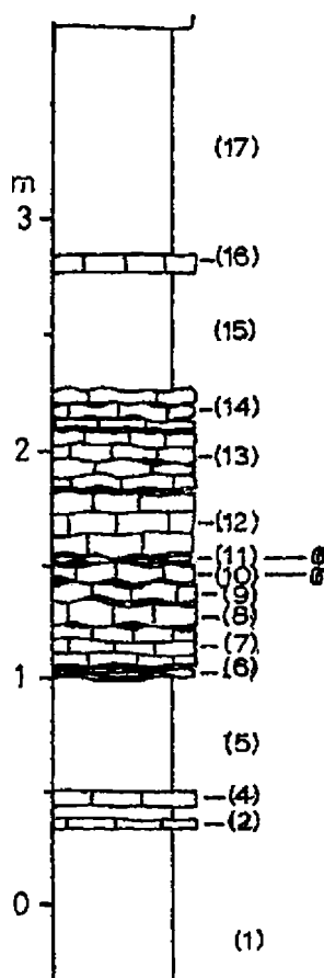
Fig. 5. Section in the Glasenbach gorge in Salzburg, a sequence of grey marls and limestones. The two limestone beds with ammonites of the Calliphyllum Zone are indicated. From other beds suitable fossils are lacking, therefore a stratigraphic subdivision of the section is not possible.
