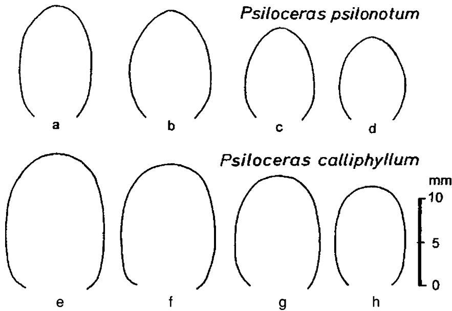
Fig. 1. Whorl sections of Psiloceras psilonotum and Psiloceras calliphyllum .
