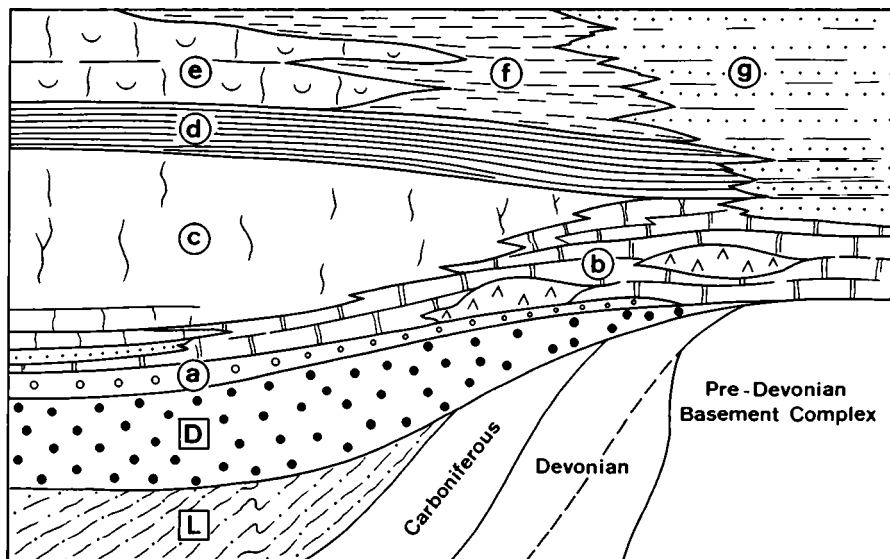
Fig. 1. Diagrammatic sketch illustrating the relationship of Permian formations in central East Greenland.
