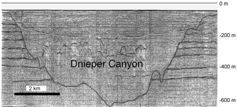
Figure 3 Cross-section of the Dniester-Dneper paleo-valley on the Ukraine shelf in a reflection profile from the 1998 BLASON survey. The valley bottom lies more than 600-m below the modern seabed, and the valley width from rim to rim approaches 10 km. The fact that the rims are just a few tens of meters below the seabed suggests that the incision and fill is young in age and not related to the Late Miocene regression 5.5 Ma ago (Hsü 1978, Hsü & Giovanoli 1979, Kojumdjieva 1983).
