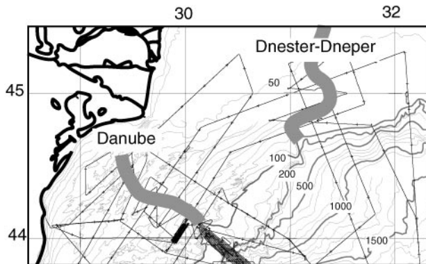
Figure 4 Paths ( stippled pattern ) of the buried Dniester-Dneper and Danube valleys mapped by seismic-reflection profiling. Bathymetric contours are light gray and are labeled in meters. Track lines are from the 1998 BLASON survey.
