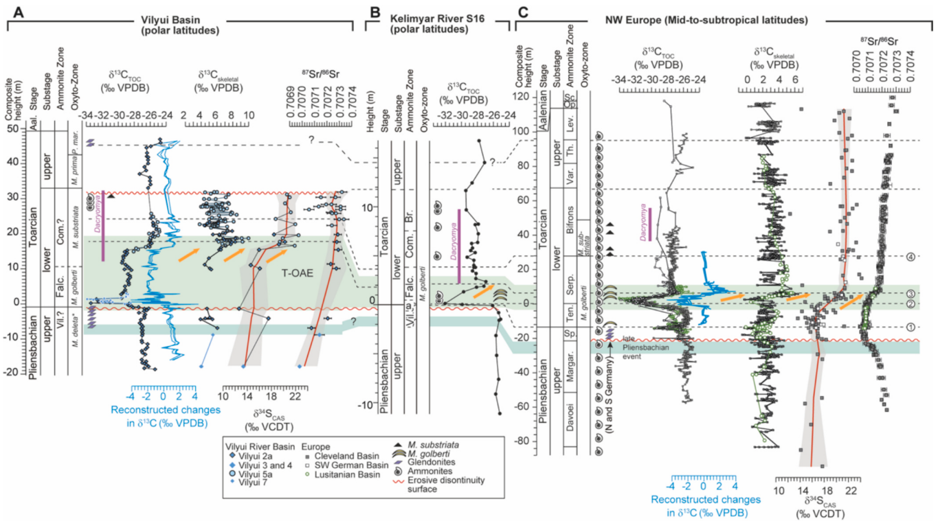
Fig. 6. Integrated stratigraphical correlations of the studied sections of Vilyui River Basin (A) with Pliensbachian–Toarcian sites of Siberia (B) (Suan et al., 2011) and Europe (C). The European \delta^{13}C_{org} (Cohen et al., 2004; Suan et al., 2015; Fantasia et al., 2019; Jenkyns et al., 2001; Trabuccho-Alexandre et al., 2022; van de Schootbrugge et al., 2020), \delta^{13}C_{skeletal} (Ferreira et al., 2019; Korte et al., 2015; McArthur et al., 2000; Suan et al., 2010, 2008; Ullmann et al., 2014), reconstructed changes in \delta^{13}C (Suan et al., 2015), \delta^{34}S_{CAS} (Gill et al., 2011; Newton et al., 2011), and \delta^{87}Sr/\delta^{86}Sr data (Jones et al., 1994a, 1994b; McArthur et al., 2000, 2020) have been projected against a composite height based on Yorkshire coast exposures. Also plotted are oxytomid bivalve Zone (Oxyto-zones) and positions of key index bivalve species from Vilyui River (this study), Kelimyar River (Lutikov, 2024; Lutikov and Arp, 2023) and Europe (Ludwigskanal); the European Dacryomya occurrence are from the Cleveland Basin (Caswell and Dawn, 2019). The European range of glendonites is based on N and S German sites (Merkel and Munneke, 2023; Teichert and Luppold, 2013). The \delta^{13}C_{org} data from Portugal (Fantasia et al., 2019) have been shifted by -3\% to compensate for terrestrial organic matter influence and facilitate reading. The red lines in the \delta^{87}Sr/\delta^{86}Sr and \delta^{34}S_{CAS} data are 50% LOESS-smoothed profiles with 95% confidence intervals (gray envelopes). Correlation lines: 1 = Pliensbachian–Toarcian boundary; 2 = base of the n-CIE; 3 = top of the n-CIE; 4 = Serpentinum–Bifrons boundary. Abbreviations: A. = Antiquium; Bra. = Braunianus; Com. = Commune Falc.; Falc. = Falciferum; Lev. = Levesquei; Op. = Opalinum; Marg. = Margaritatus; Sc. = Scissum; Serp. = Serpentinum; Sp. = Spinatum; Ten. = Tenuicostatum; Th. = Thouarsense; Var. = Variabilis; Vil. = Vilgaensis; (For interpretation of the references to colour in this figure legend, the reader is referred to the web version of this article.)
