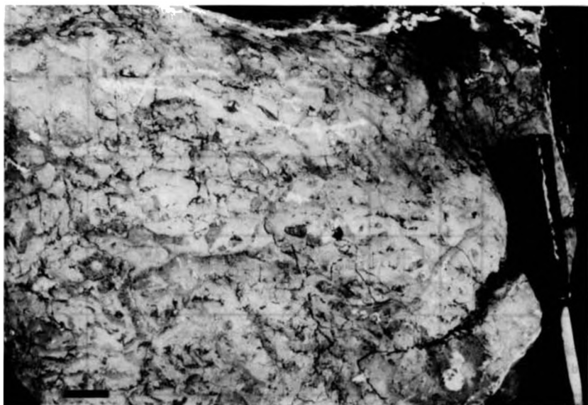
Fig. 8. Siliceous sponge meadow facies (facies type 1c). Platy "lithistid" sponges are embedded in a micritic matrix. Microbial crusts occur subordinately. Length of bar is 4 cm. Tavira quarries, eastern Algarve.
