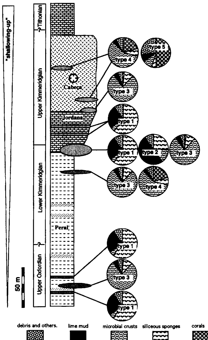
Fig. 21. Generalized composite section of the Upper Jurassic succession in the eastern Algarve. The succession represents a clear shallowing-upwards trend from ammonite marls (Peral) to allochthonous intraclastic bioclastic limestones (Jordana) to coral platform facies (Cabeça) to lagoonal biomicrites. Note that coral-rich siliceous sponge facies (types 4, 5) is restricted to the upper part, whereas thrombolites (type 3) and siliceous sponge meadows (type 1) occur over a wide range.
