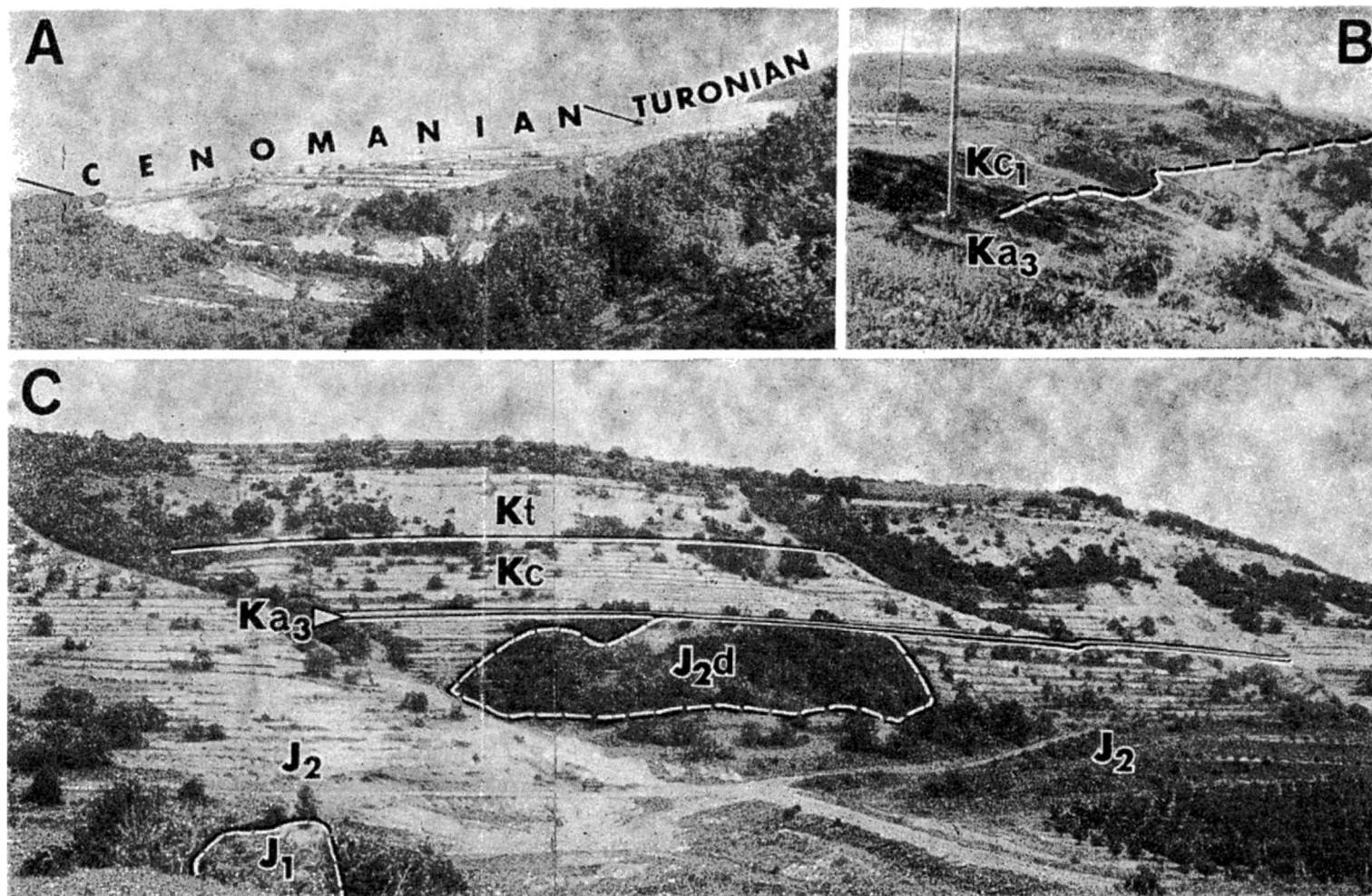
Exposures of the Upper Albian, Cenomanian and Turonian deposits in SW Crimea Highland, Soviet Union
