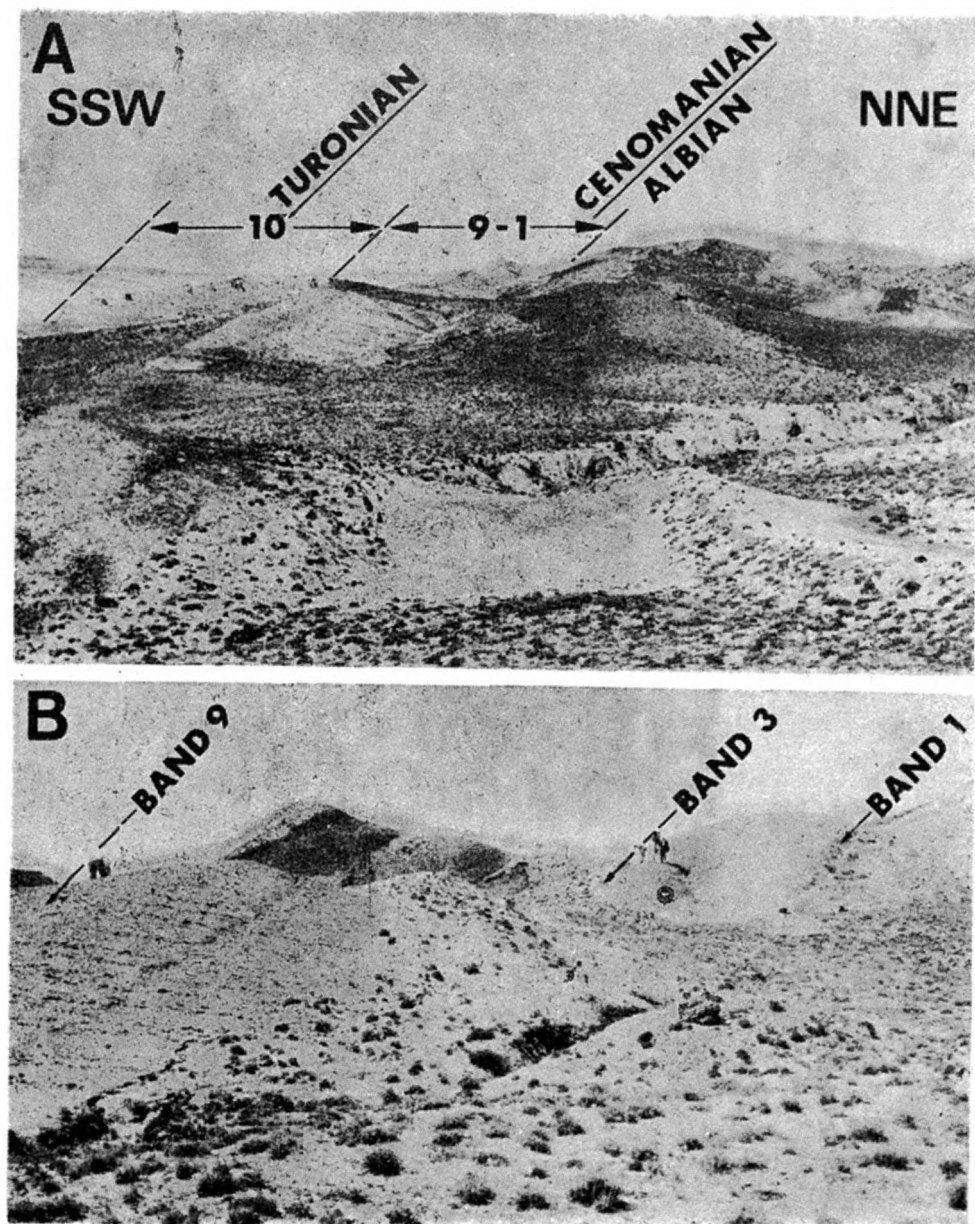
Exposures of the Albian, Cenomanian and Turonian deposits in the Sullu-kapy section, Mangyshlak, Soviet Union
