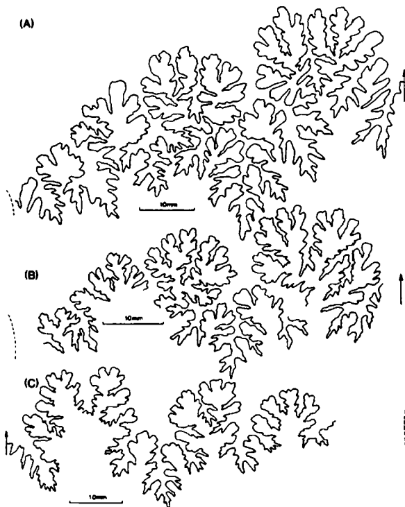
TEXT-FIG. 2. Suture lines of A, Euhoploceras ( Fissiloboceras ) fissilobatum (Waagen), HMS 15343/3 at Wh 69.3 mm ( \times 1.3 ); B, Euhoploceras ( Fissiloboceras ) fissilobatum (Waagen), HMS 15343/4 at Wh 60.9 mm ( \times 1.4 ); C, Shirbuirnia trigonalis Buckman, HMS 15342/1 at Wh 75.2 mm ( \times 1.2 ).
