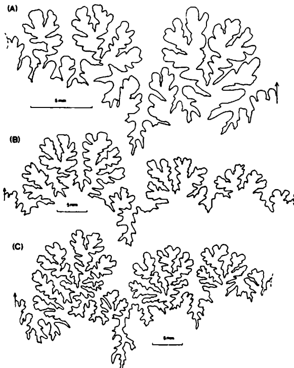
TEXT-FIG. 8. Suture lines of A, Sonninia (Papilliceras) arenata (Quenstedt), HMS 15341/2 at Wh 22.3 mm ( \times 3.8 ); B, Sonninia (Papilliceras) arenata (Quenstedt), HMS 15341/3 at Wh 40.2 mm (Quenstedt), HMS 15341/3 at Wh 40.2 mm ( \times 1.8 ); C, Sonninia (Papilliceras) mesacantha (Waagen), HMS 26420/1 at Wh 38.5 mm ( \times 1.8 ).
