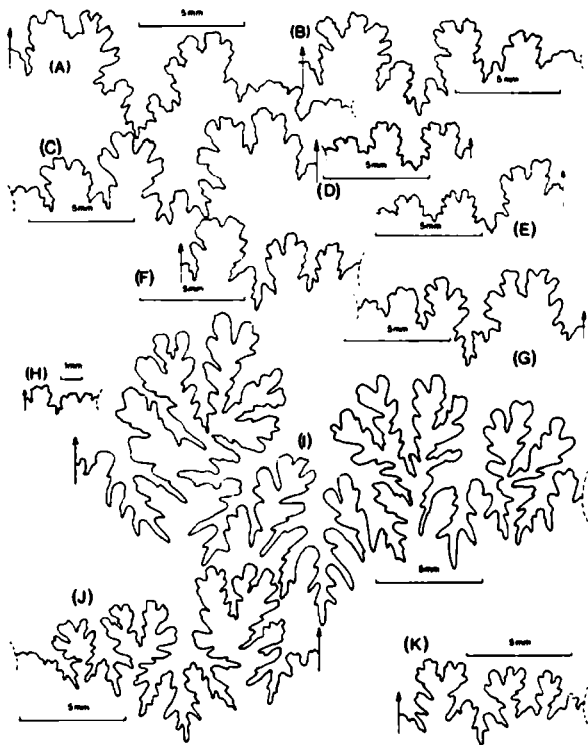
TEXT-FIG. 5. Suture lines (all < 3.4 ) of A, Witchellia aff. rubra (Buckman), HMS 15346/2 at Wh 16.1 mm; B, Witchellia aff. rubra (Buckman), HMS 26404/8 at Wh 13.8 mm; C, Witchellia aff. romanoides (Douville), HMS 26408 at Wh 13.6 mm; D, Pelekodites zurcheri (Douville), HMS 26409/1 at Wh 6.0 mm; E, Pelekodites zurcheri (Douville), HMS 26410/1 at Wh 7.9 mm; F, Pelekodites macer (Buckman), HMS 15340/14 at Wh 7.6 mm; G, Pelekodites macer (Buckman), HMS 26412/14 at Wh 8.1 mm; H, Pelekodites minimus (Hiltermann), HMS 26413/2 at Wh 3.2 mm; I, Sonninia ( Sonninia ) cf. propinquans (Bayle), GSE 3060 at Wh 21.2 mm; J, Sonninia ( Sonninia ) corrugata (Sowerby), HMS 15345/1 at Wh 13.0 mm; K, Sonninia ( Sonninia ) corrugata (Sowerby), HMS 15345/2 at Wh 8.2 mm.
