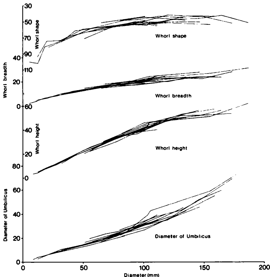
TEXT-FIG. 7. Umbilical diameter, whorl height, whorl breadth, and whorl shape plotted against diameter for specimens of Sonninia (Papilliceras) arenata (Quenstedt) from Skye.
