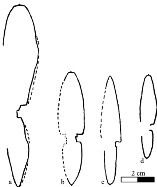
Fig. 16: Streblites weinlandi (OPPEL, 1863) [M], whorl sections, \times 1 ; a: specimen No. crl126, coll. BAUDOUIN; b: specimen No. crl055, coll. BAUDOUIN; c: specimen No. crl060, coll. BAUDOUIN; d: specimen No. crl072, coll. BAUDOUIN.
