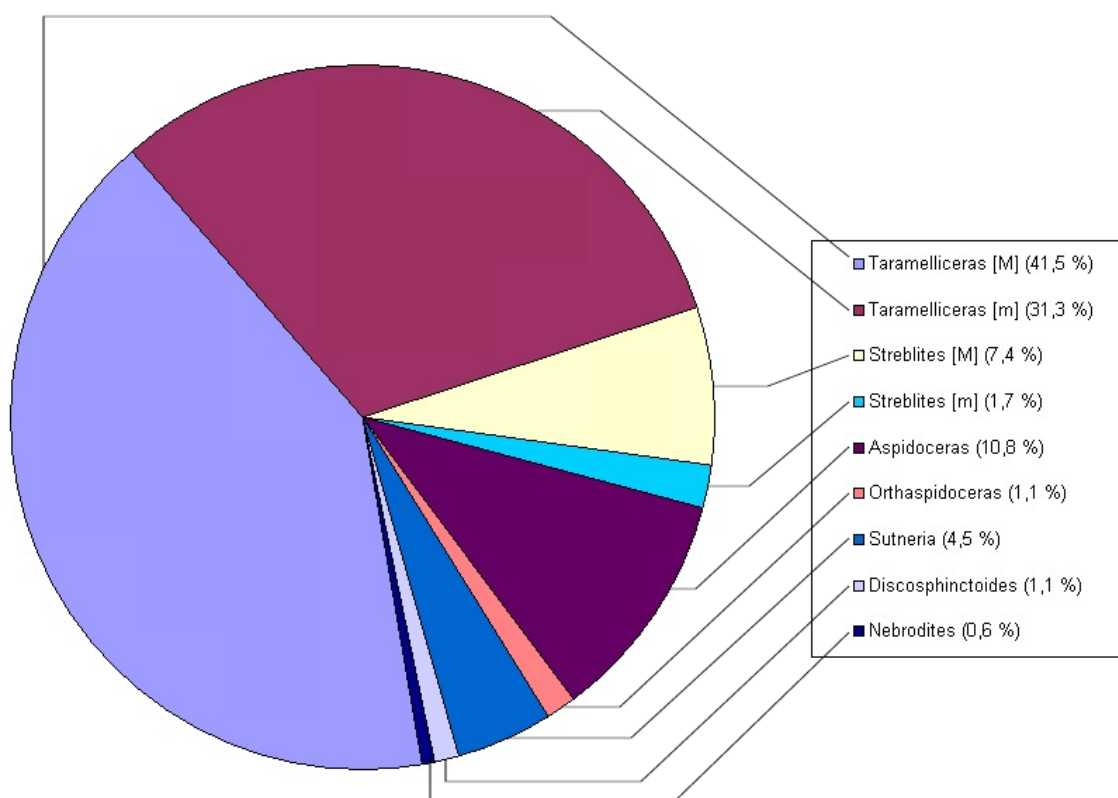
Fig. 7: The ammonites' genera in bed No. 195 (N=176).
