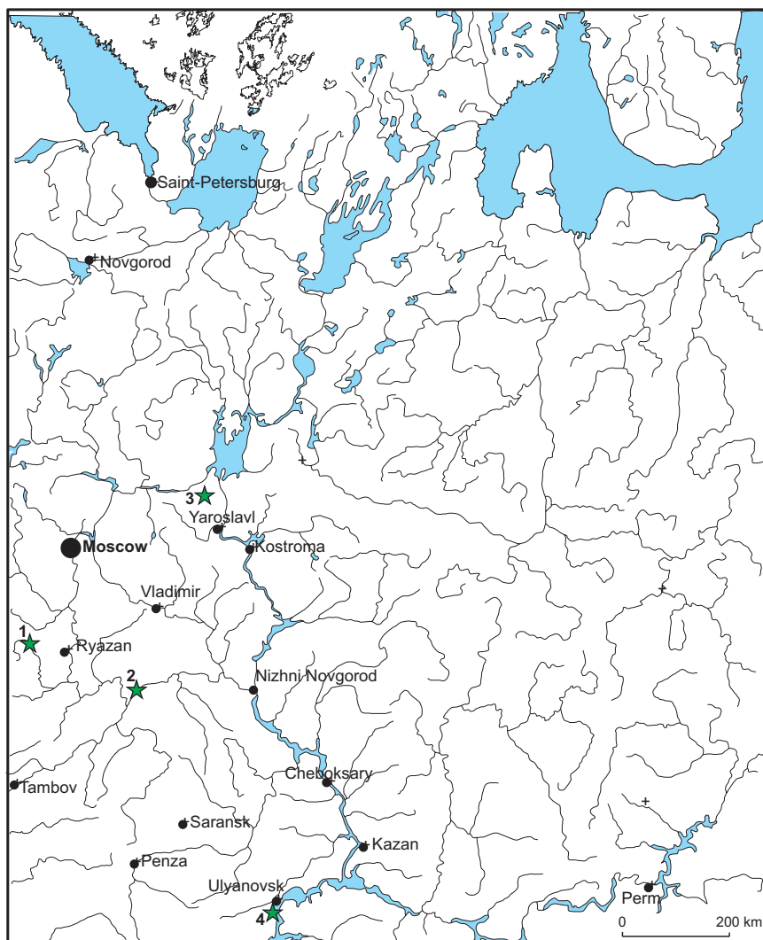
Fig. 2. Map showing mentioned localities of the Russian Platform
